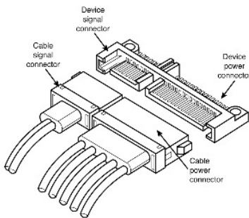
Figure 2. Attaching SATA cabling
