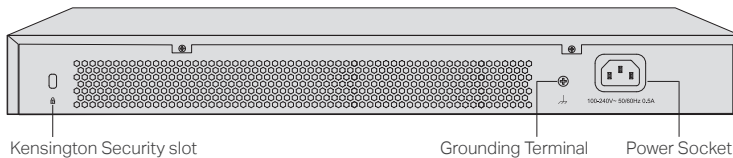
Figure 1-10 Rear Panel
